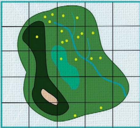
1. Random Sampling
