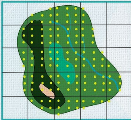
3. Systematic Sampling
